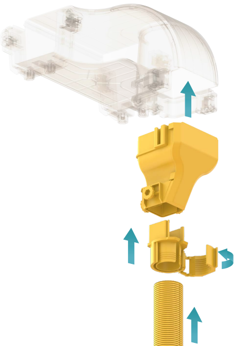
Reducer to R3 Tube Assembly
